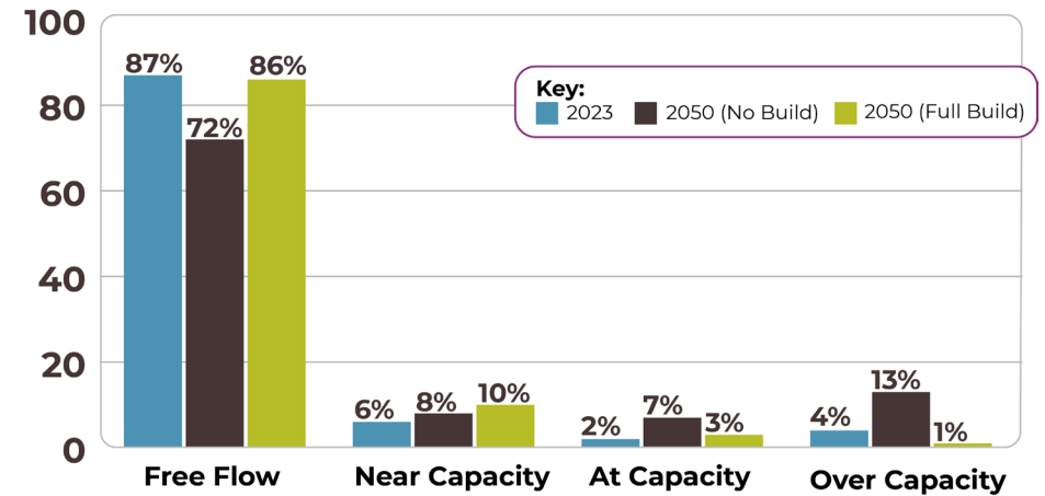
Figure 14: Current and Future Volume-to-Capacity
